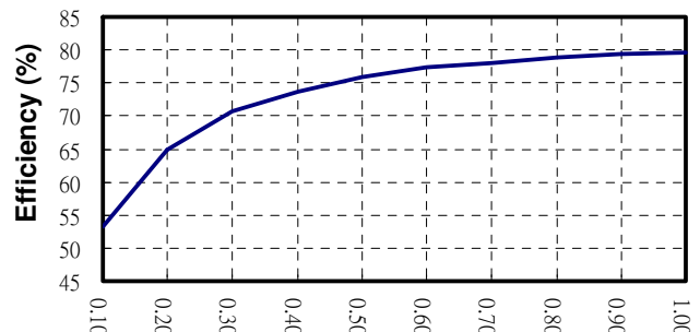
Output Current vs. Efficiency
