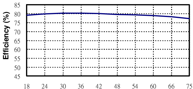
Input voltage vs. Efficiency
